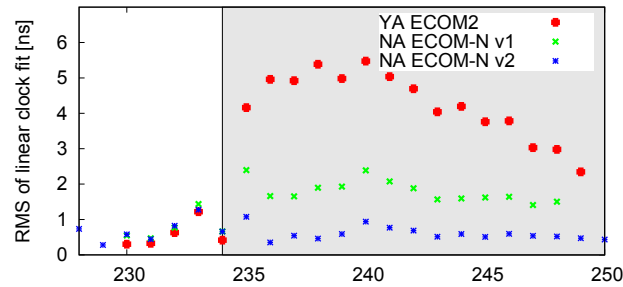
Figure 6: RMS of daily linear fit through epoch-wise satellite clocks of QZS-1 between DOY 228 and 250/2015. Gray background: Satellite is in orbit normal mode. YA: Yaw attitude law applied. NA: Normal attitude law applied. ECOMx: SRP model version.
