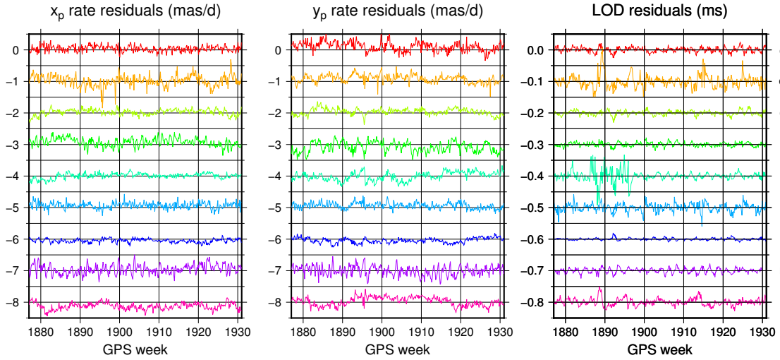
Figure 3: AC pole rate and LOD residuals from the 2016 daily IGS SINEX combinations. The individual AC time series have been shifted by multiples of 1 mas/d and 0.1 ms for clarity.
