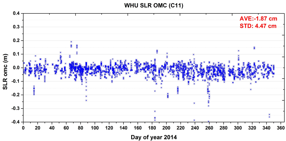
Figure 6: Beidou C11 orbit validation by SLR.
