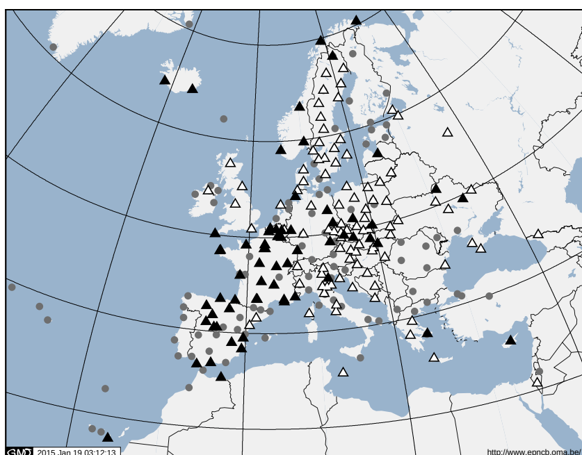
Figure 2: EPN tracking stations capable of tracking L5 indicated with △; those in addition including L5 in their RINEX v2.11 data are indicated by ▲ (status in December 2014).
