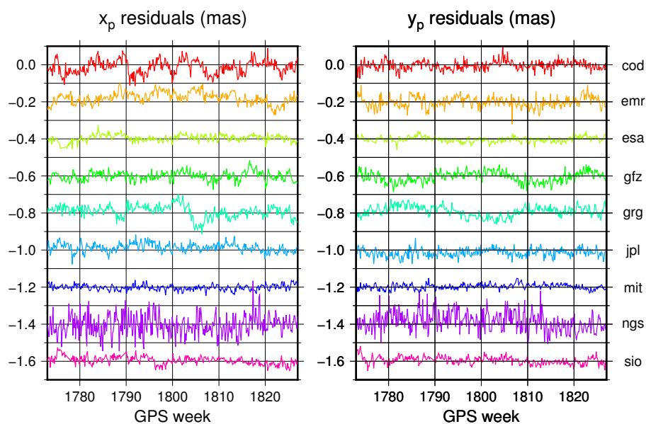
Figure 2: AC pole coordinate residuals from the 2014 daily IGS SINEX combinations. The individual AC time series have been shifted by multiples of 0.2 mas for clarity.
