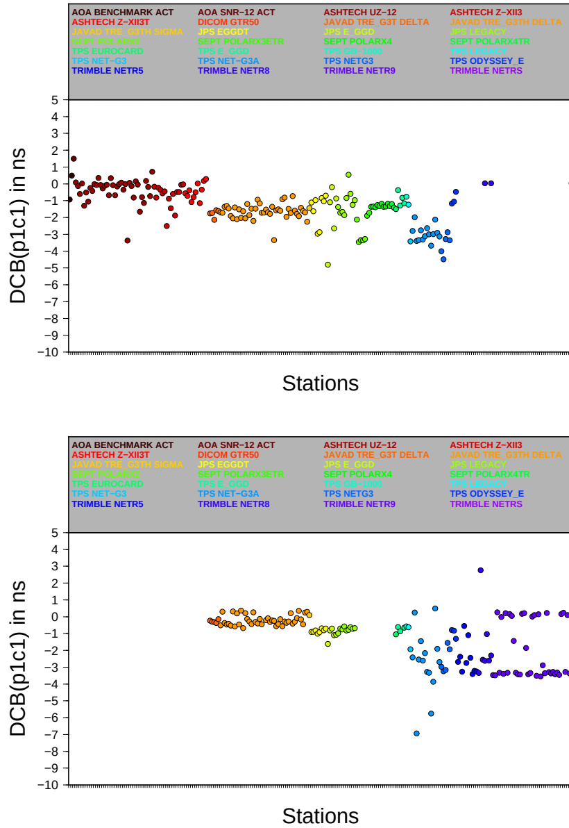
Figure 5: Monthly set of P1-C1 differential code biases for the GPS (top) and GLONASS (bottom) receiver components, for December 2014, computed at CODE.
