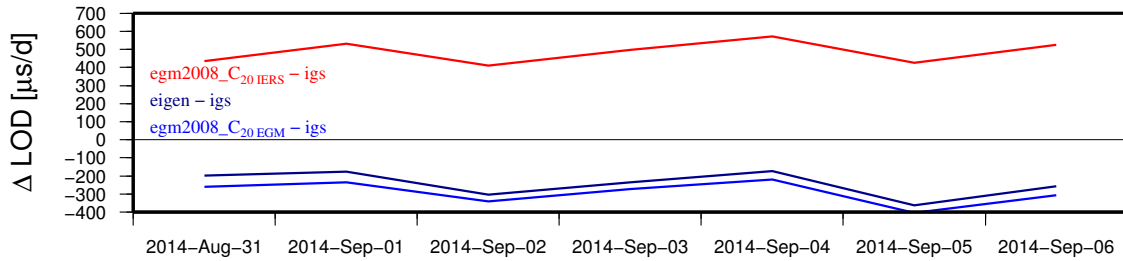
Figure 3: Differences in length of day (LOD) estimates with respect to IGS Final combined LOD product (igs) based on different internal GFZ solutions. eigen: EIGEN_GL04C gravity model, egm2008_C 20 IERS: EGM2008 gravity model but with supplemented IERS2010 C 20 -term (from Tab. 6.2 in Petit and Luzum 2010); egm2008_C 20 EGM: EGM2008 gravity model.
