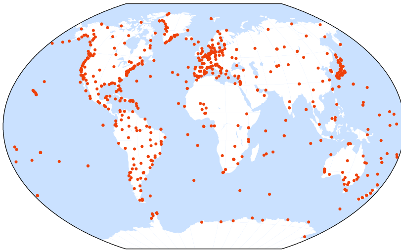
Figure 1: GPS network processed at BLT for TIGA.
