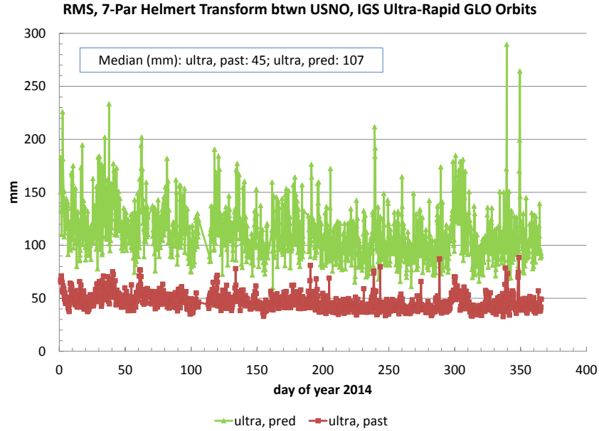
Figure 5: RMS of USNO ultra-rapid GLONASS orbit estimates with respect to IGS Combined Ultra-rapid GLONASS orbits, 2014. “Ultra, past” refers to 24-hour post-processed section of USNO ultra-rapid orbits. “Ultra, pred” refers to first six hours of ultra-rapid orbit prediction. Helmert transformations computed using Bernese 5.0 Software .
