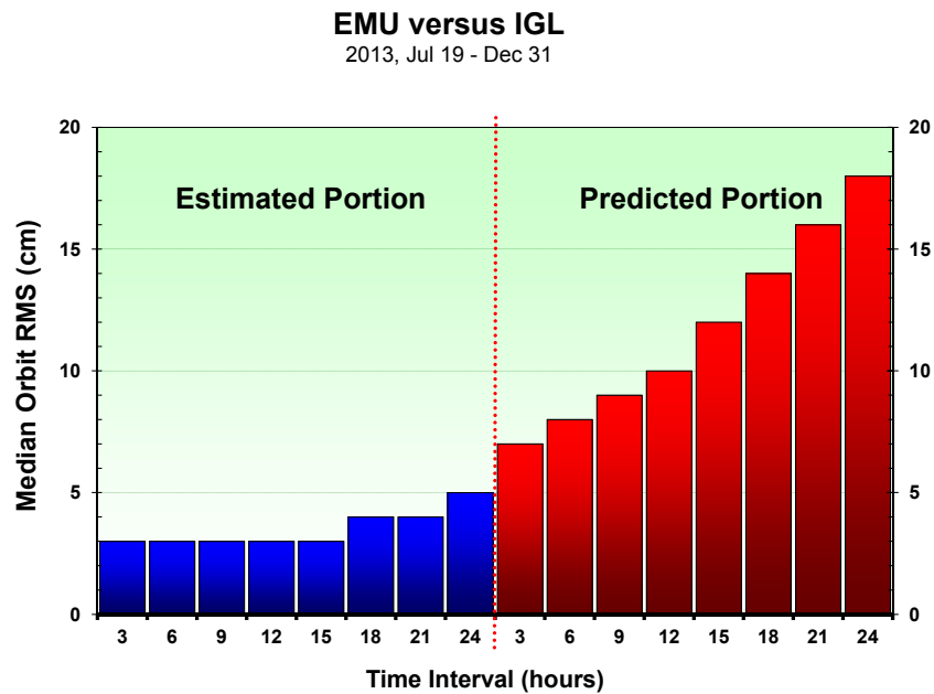
Figure 2: GLONASS Ultra-Rapid Orbit Median RMS for 2013.
