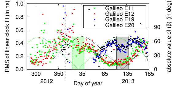
Figure 7: RMS of daily linear fit through estimated epoch-wise Galileo satellite clocks (big dots). The shaded areas mark the eclipsing seasons of E11, E12 (green) and of E19, E20 (black). The curves show the absolute value of the elevation of the Sun w.r.t. the satellite's orbital planes ( \beta ) with the same color code as the boxes.
