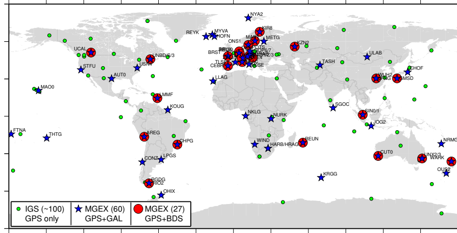
Figure 3: Global network of IGS (green) and MGEX stations, which were set up for data processing. The 60 Galileo–MGEX stations (blue) realize a good global coverage for practical Galileo orbit determination purposes, whereas a lot of the 27 BeiDou–MGEX stations (red) are concentrated in Europe.
