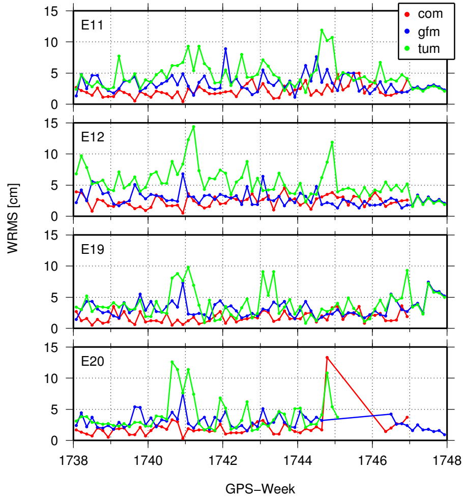
Figure 4: Weighted RMS (WRMS) of individual MGEX-AC orbits with respect to the combined result for all Galileo-IOV satellites (Note: E20 out-of-service around GPS-week 1745)
