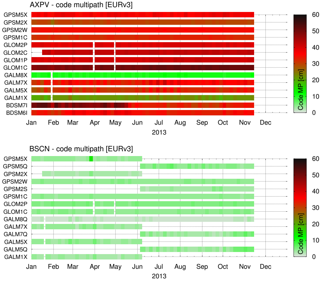
Figure 1: Pseudorange multipath estimated for all GNSS signals observed at the EUREF station AXPV (top) and BSCN (bottom) during January–November, 2013
