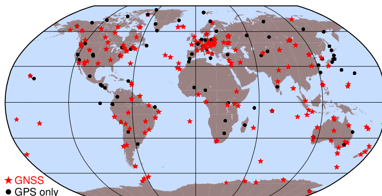
Figure 1: Network used for the GNSS final processing at CODE by the end of 2013.
