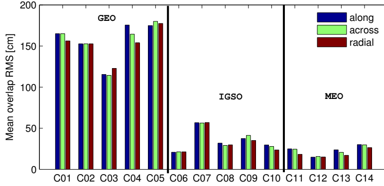
Figure 6: Mean orbit overlap RMS[cm] in along, across and radial.
