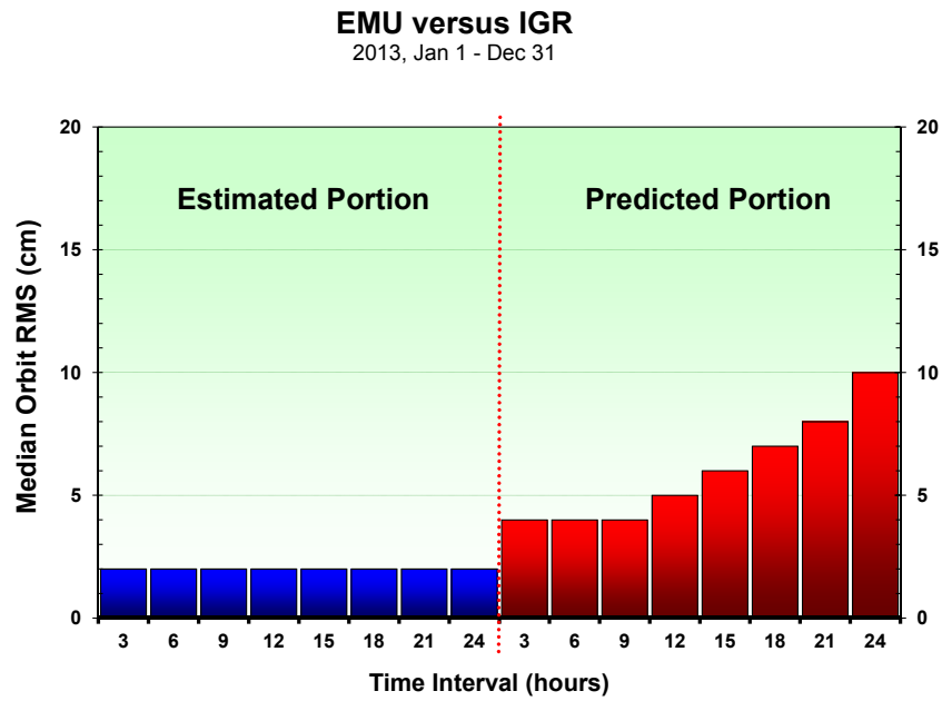
Figure 1: GPS Ultra-Rapid Orbit Median RMS for 2013.
