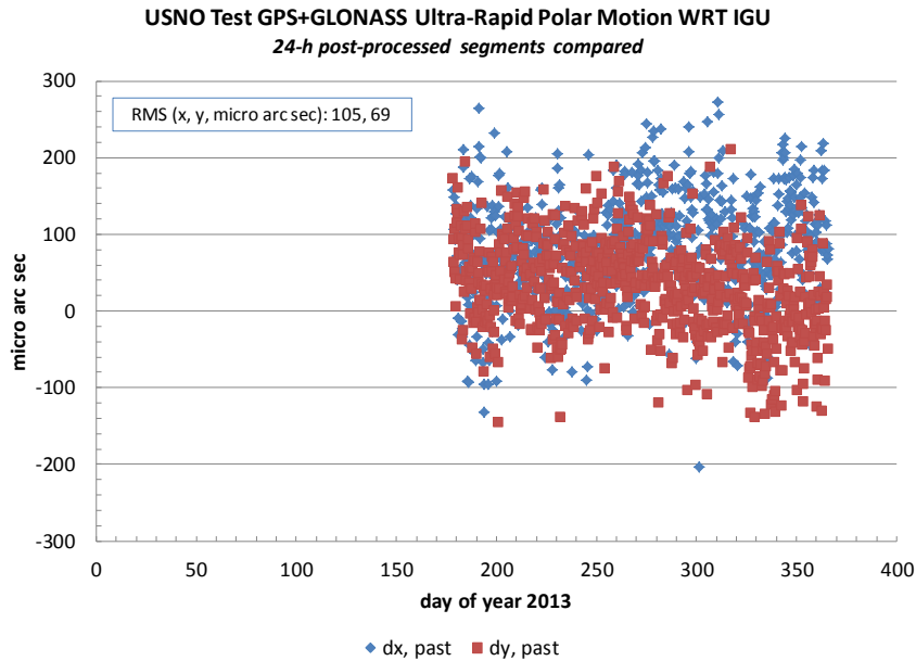
Figure 6: Difference between 24-h post-processed polar motion estimates in USNO test ultra-rapid GPS+GLONASS solution and IGS “IGU” GPS-only ultra-rapid solution, 2013.
