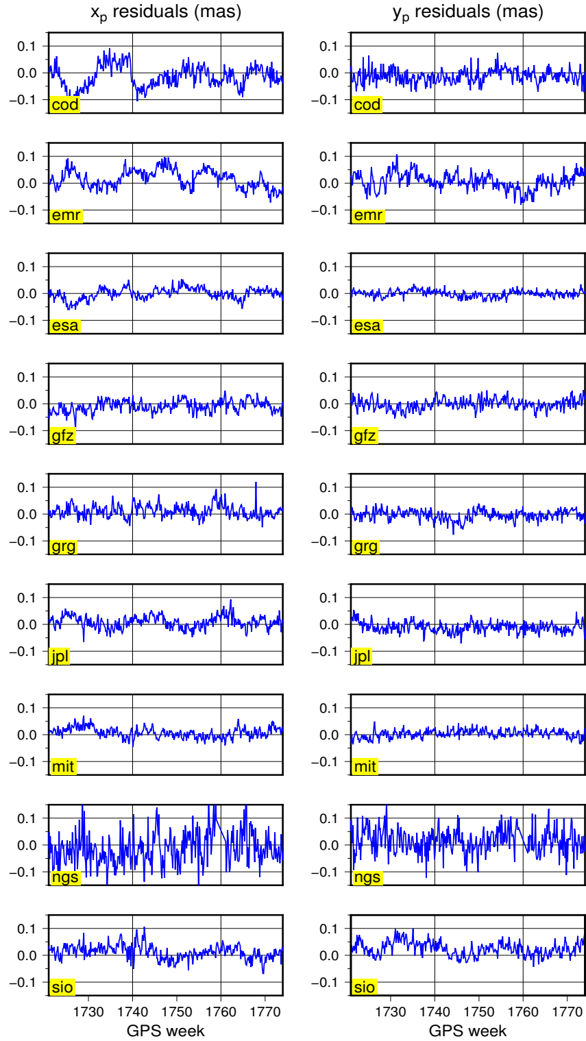
Figure 2: AC pole coordinate residuals from the 2013 daily IGS SINEX combinations.
