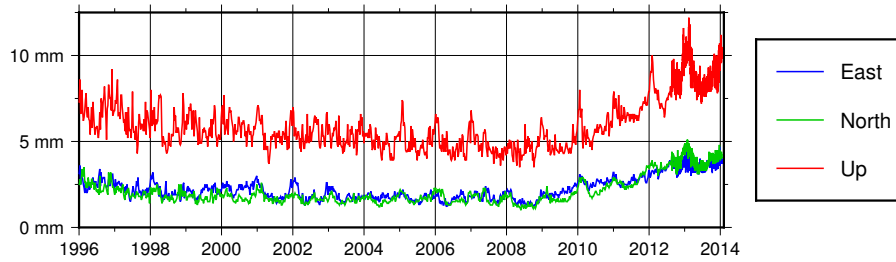
Figure 6: RMS of the residuals from 7-parameter similarity transformations between the weekly/daily IGS combined solutions and the IGS08/IGb08 Reference Frames. The igb weekly solutions (IGSMAIL #6401) were used for the period before GPS week 1632. The operational IGS combined solutions were used afterwards.
