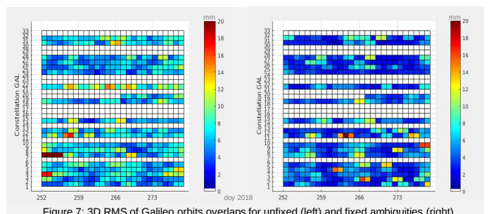
Figure 7: 3D RMS of Galileo orbits overlaps for unfixed (left) and fixed ambiguities (right)
